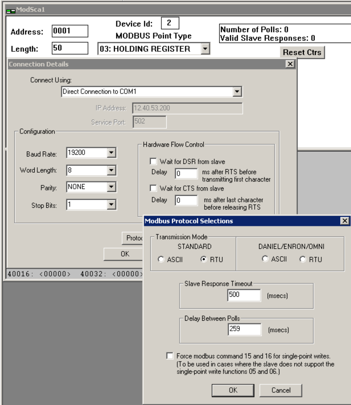
Figure 7.14: ModScan32 Master Scanning Program Serial Connection Setup, select RTU or ASCII Transmission Mode.
